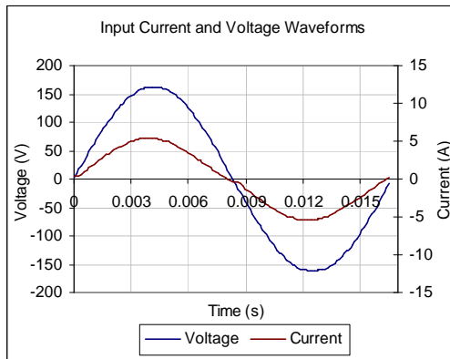
Input AC Current Waveform (ITHD = 11.96%, 50% Load)
